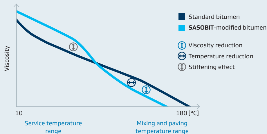
Viscosity curves of standard bitumen and SASOBIT -modified bitumen
